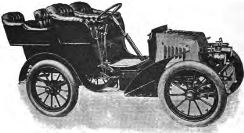
FIG. 408.—One model of the "Peerless" Gasoline Carriage, equipped with wooden wheels and removable tonneau.
